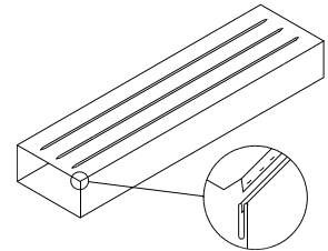
Button Lock Duct
