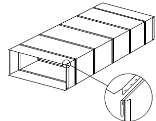
Cleat Fold Duct
