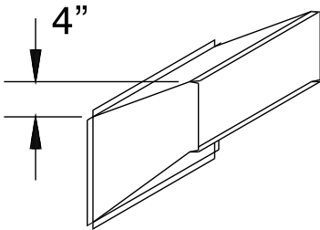
Plenum Take Off — 4" Rise
