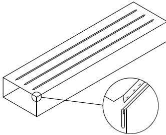
Button Lock Duct
