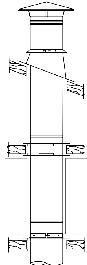
Type B Gas Vent Pipe and Fittings
